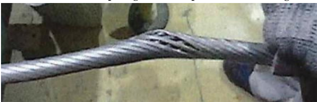
(single hook hoisting with tension)
